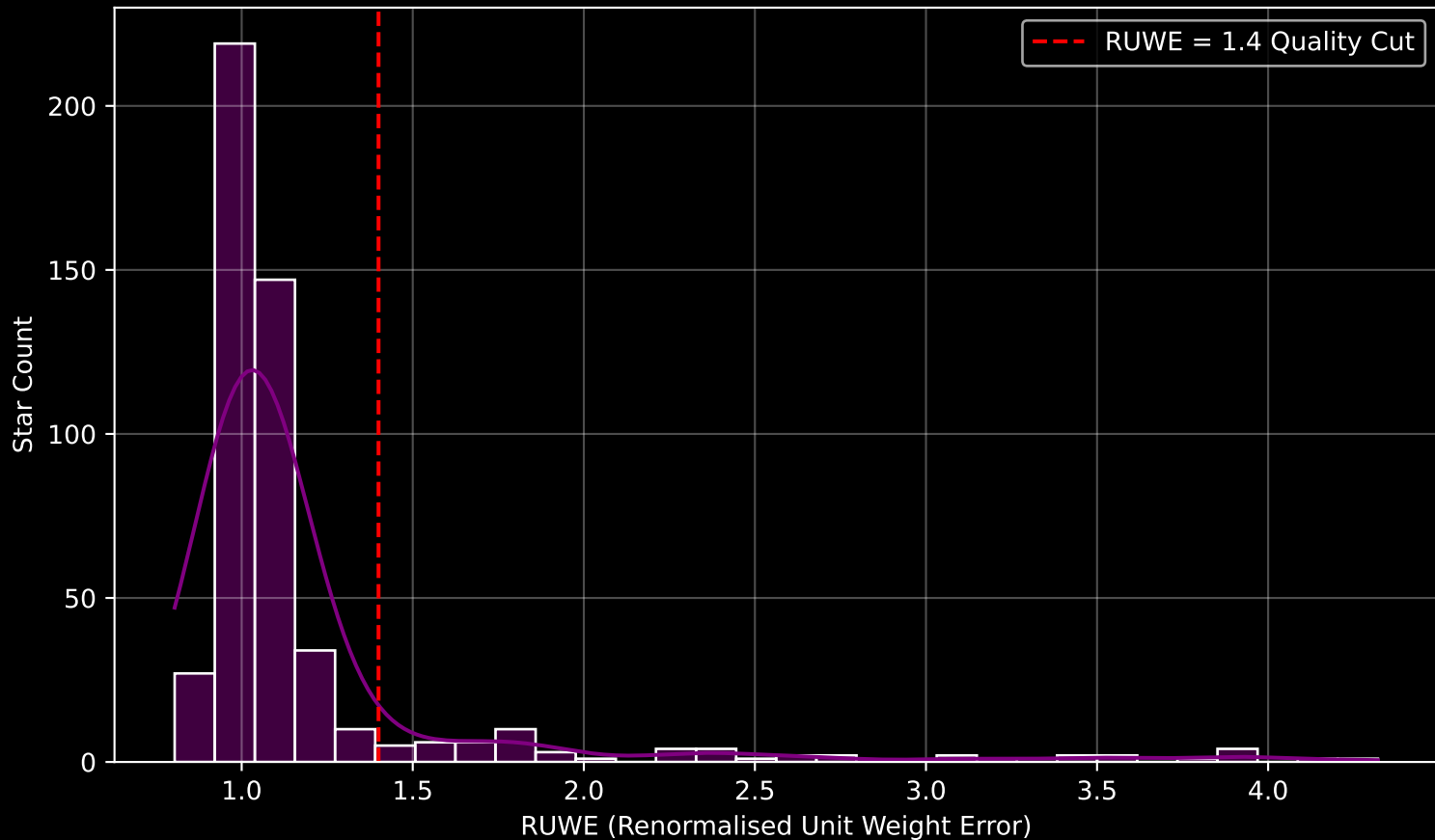
GALAH DR4 Field [6777] RUWE Distribution (n= 495)
