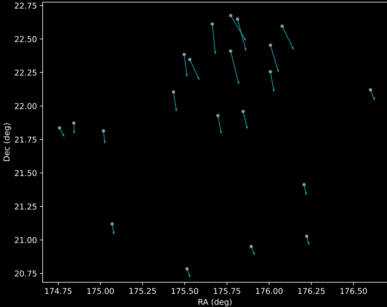
GALAH DR4 Cluster 18 Proper Motion Vectors (n=21)
