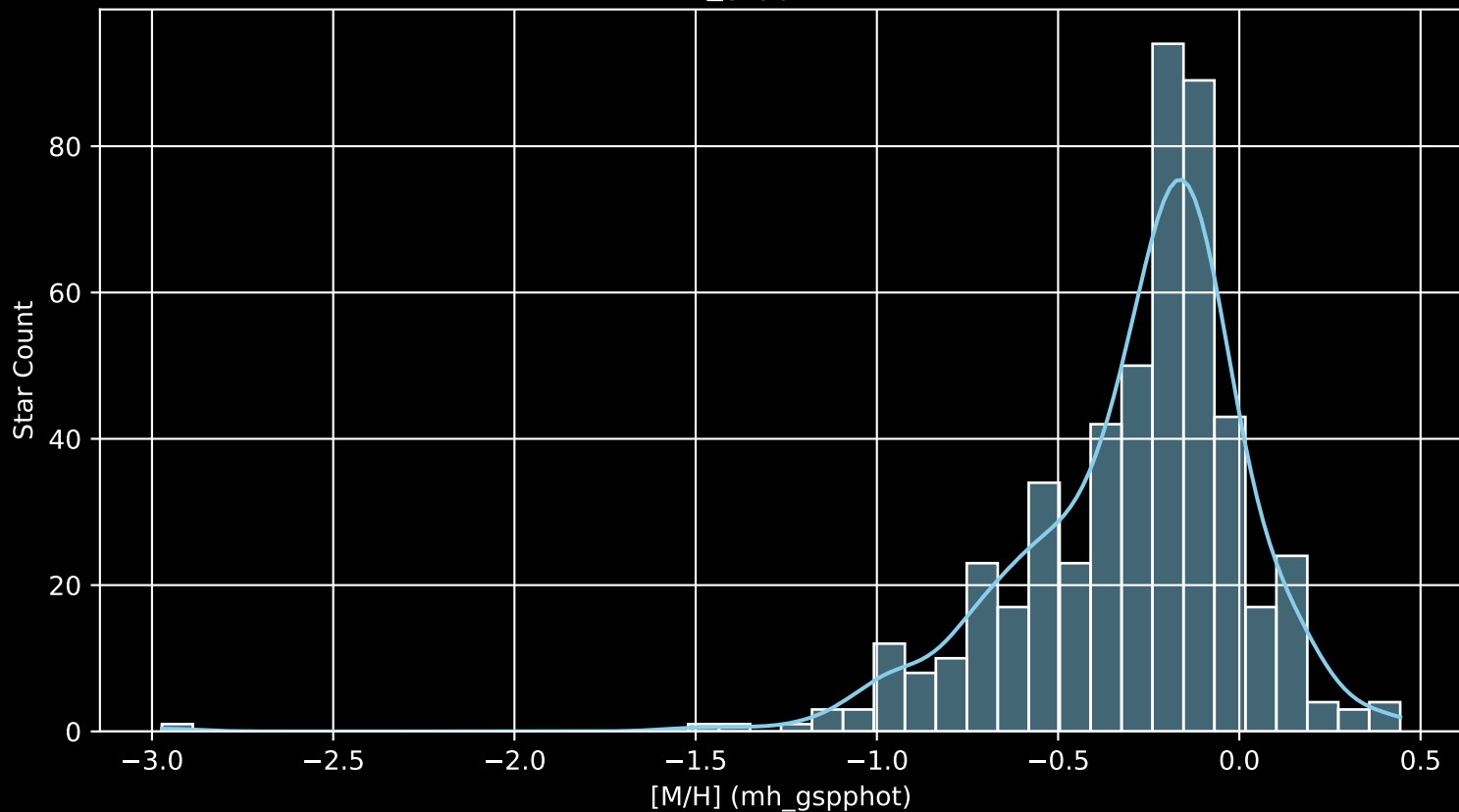
GALAH DR4 Field: [6777] [M/H] (mh_gspphot) (n= 507)
