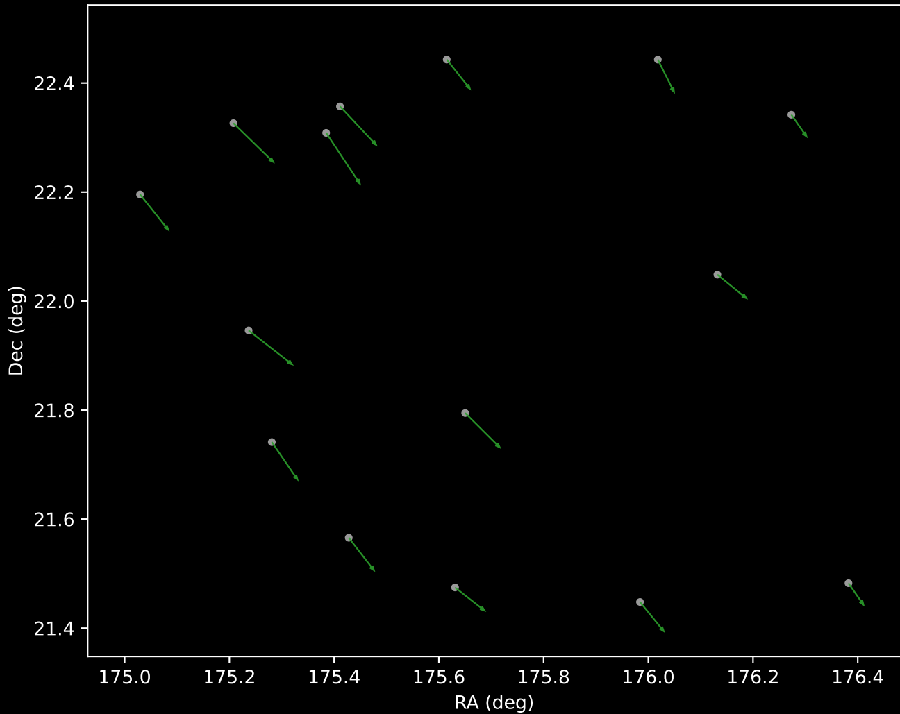
GALAH DR4 Cluster 24 Proper Motion Vectors (n=15)
