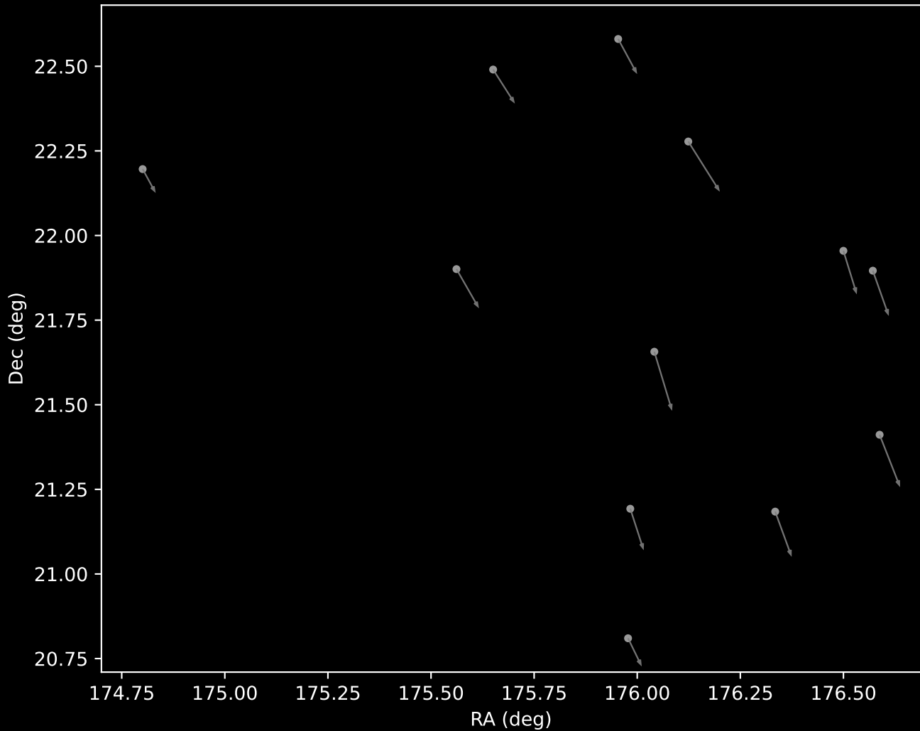
GALAH DR4 Cluster 14 Proper Motion Vectors (n=12)
