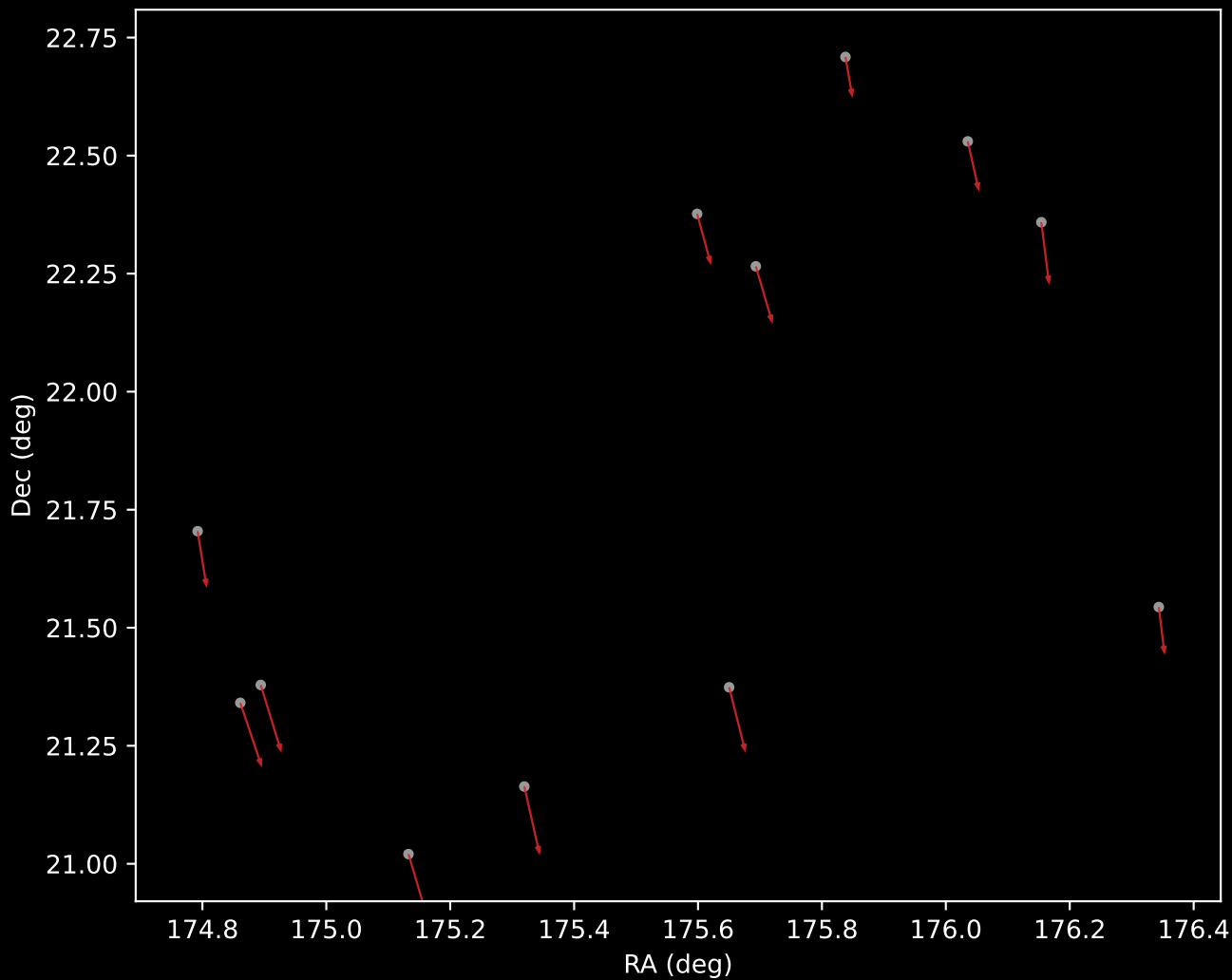
GALAH DR4 Cluster 26 Proper Motion Vectors (n=12)
