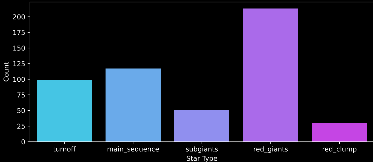
GALAH DR4 Field: [6777] Count plot of Star Type
