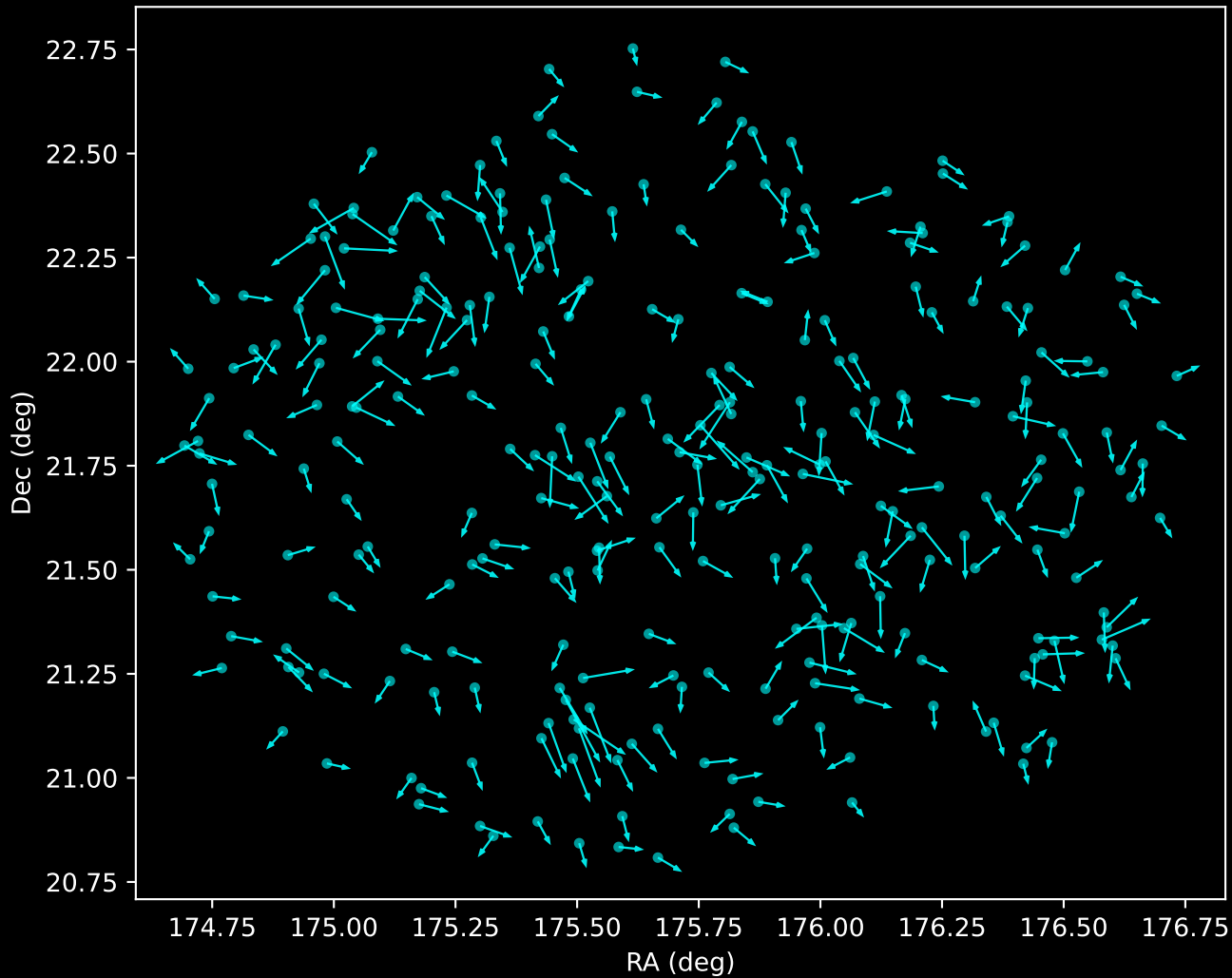
GALAH DR4 Noise Stream Proper Motion Vectors (n=279)
