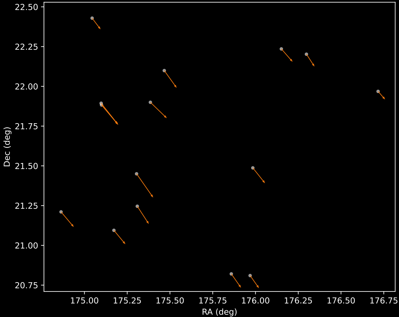
GALAH DR4 Cluster 22 Proper Motion Vectors (n=15)
